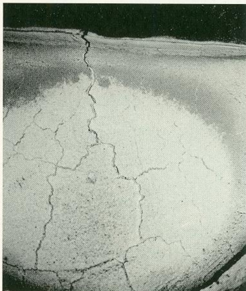
Surface cracks on ceramic fiber refractory
